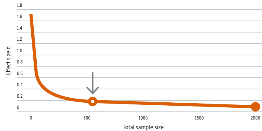
FIGURE 5: THE POWER TO DETECT AN EFFECT BETWEEN TWO CONDITIONS IN A BETWEEN-SUBJECT DESIGN WITH THE THRESHOLD FOR SIGNIFICANCE AT P < 0.05 (ONE-TAILED) 9
