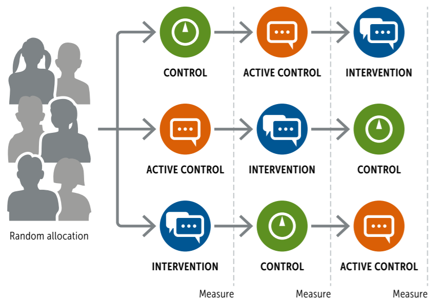
FIGURE 4: A WITHIN-SUBJECT DESIGN WITH THREE CONDITIONS (WITH COUNTERBALANCING)
