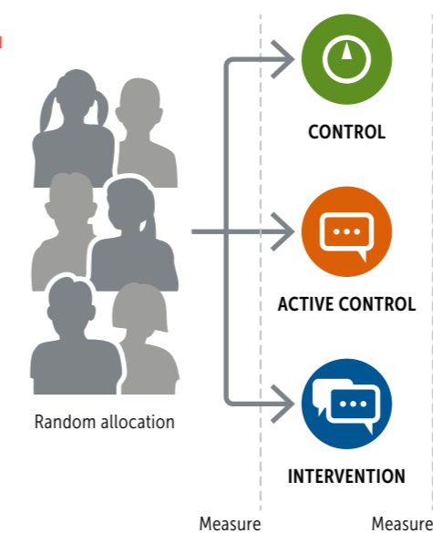
FIGURE 3: A BETWEEN-SUBJECT DESIGN WITH THREE CONDITIONS
